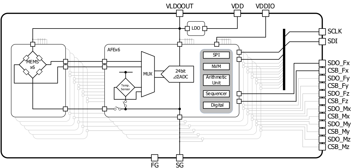
Fig. 3 Block Diagram
