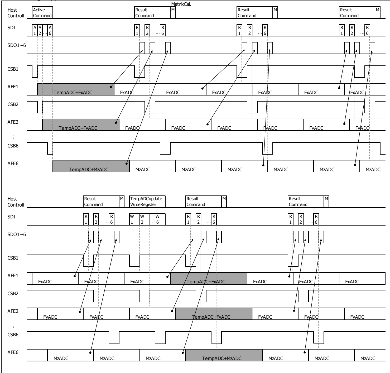
*AD conversion cycle depends on AFE because internal clock is different from each AFE. Fig. 18 Common to SDO pin - Measurement timing chart
