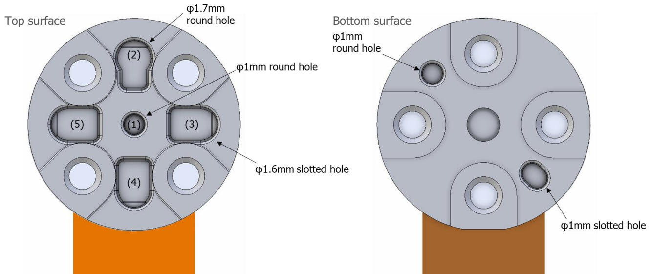
Fig. 35 Positioning holes
