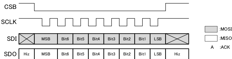
Fig. 20 SPI Waveform
